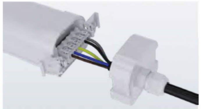
5-core Terminal
