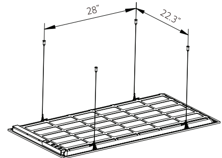
DPS-PKT-14-S 4-Cable Kit
