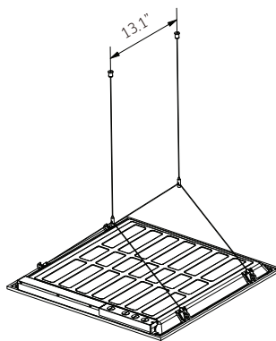
DPS-PKT-12-S 2-Cable Kit
