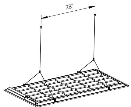
DPS-PKT-12-S 2-Cable Kit
