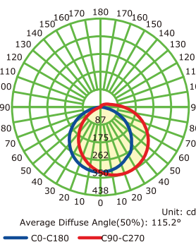
Luminous Intensity Distribution Curve
