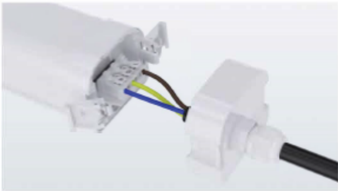
3-core Terminal
