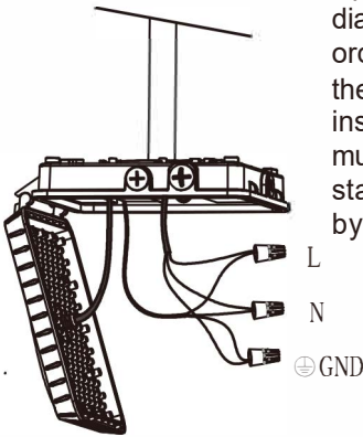
Figure 1. Wiring Diagram
