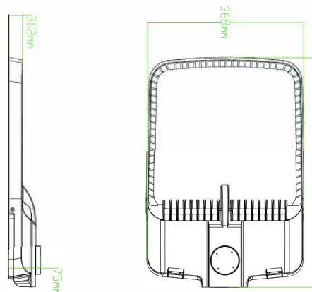
SIZE 368x541x75mm Max 320W
