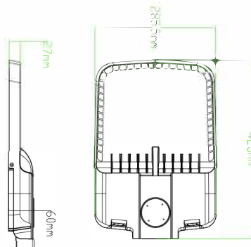
SIZE 285x523x60mm Max 180W
