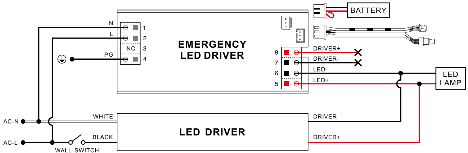
FIG B. FOR LED LUMINAIRE > 120W or > 3A LED DRIVER CURRENT.
